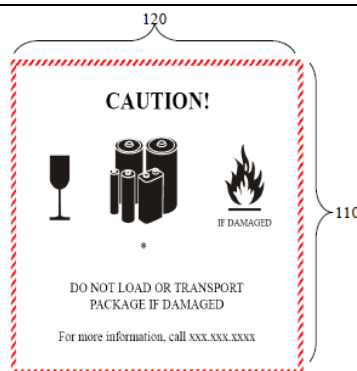
Figure 3 lithium battery handling label
